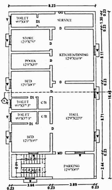
EXISTING GROUND FLOOR PLAN
