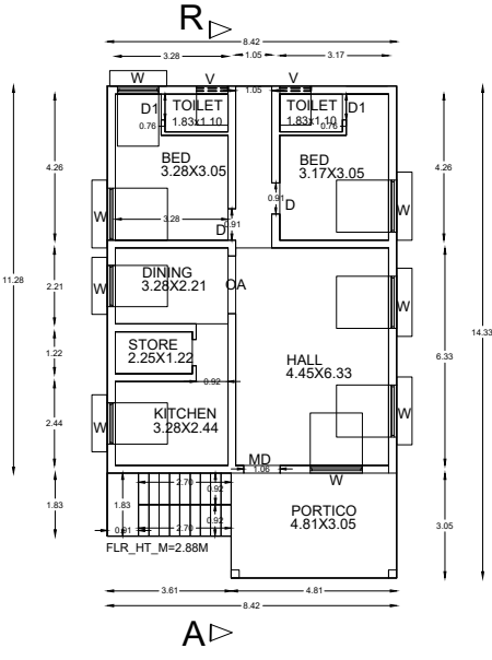
GROUND FLOOR PLAN=0
