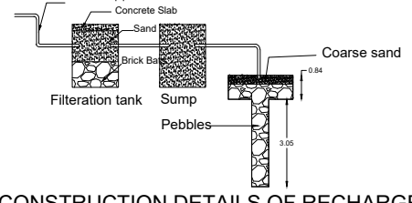
CONSTRUCTION DETAILS OF RECHARGE TRENCH
