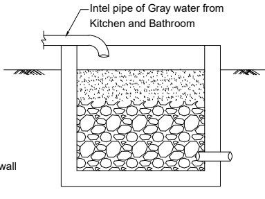
GREY WATER RECYCLING CHAMBER:-
