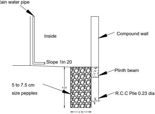
RAIN WATER COLLECTION TRENCH:- NOT TO SCALE
