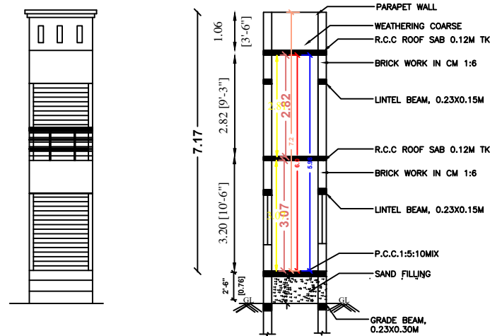
ELEVATION SECTION ON A A
