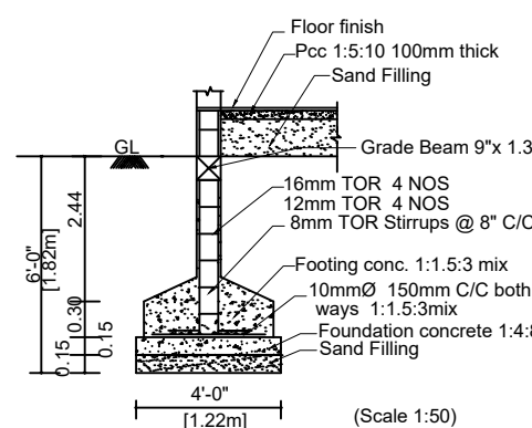
FOUNDATION DETAILS
