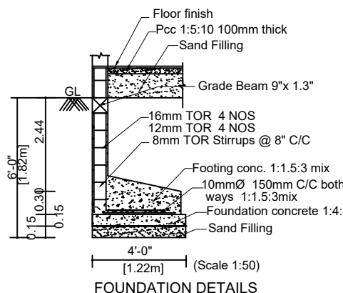
FOUNDATION DETAILS
