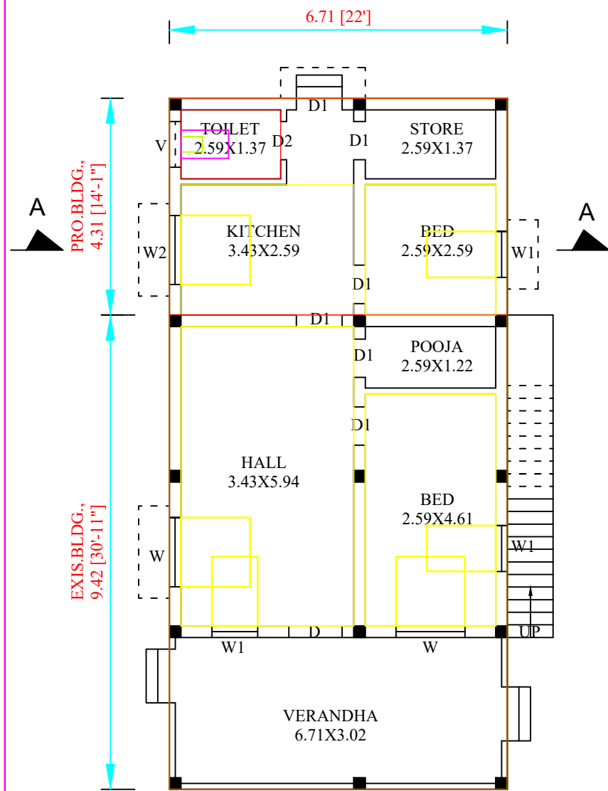
PRO.ADD.GROUND FLOOR PLAN
