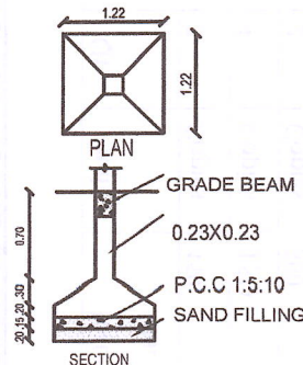
FOUNDATION DETAILS
