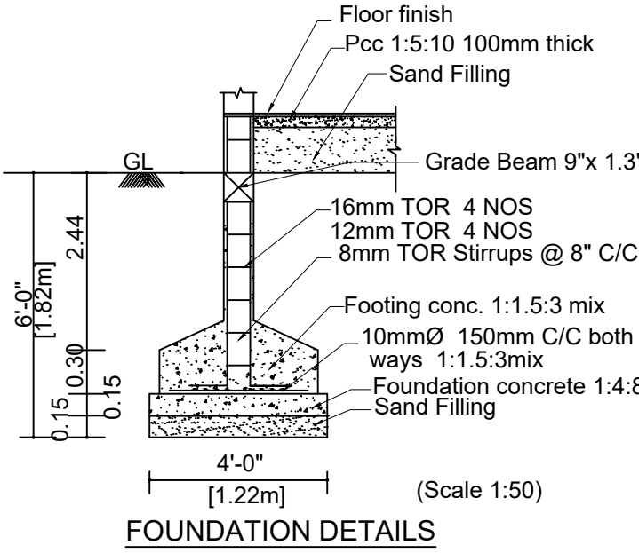
FOUNDATION DETAILS
