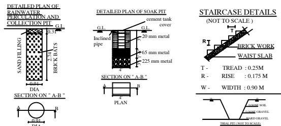
STAIRCASE DETAILS (NOT TO SCALE)
