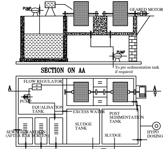
PLAN SEWAGE TREATMENT PLANT DETAILS
