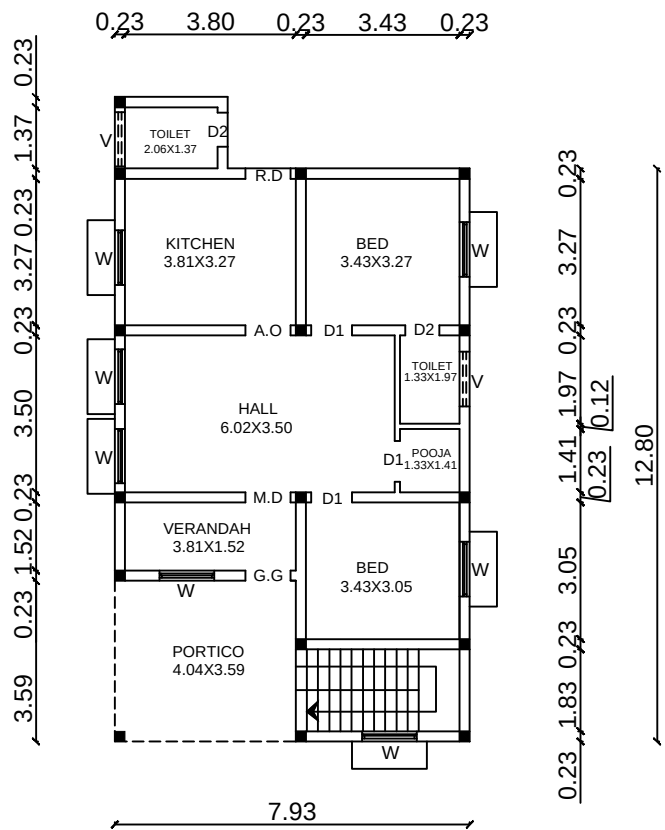
FLOOR GROUND
