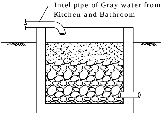
GREY WATER RECYCLING CHAMBER:-
