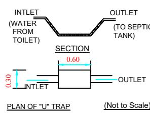
PLAN OF "U" TRAP (Not to Scale)
