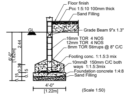
FOUNDATION DETAILS
