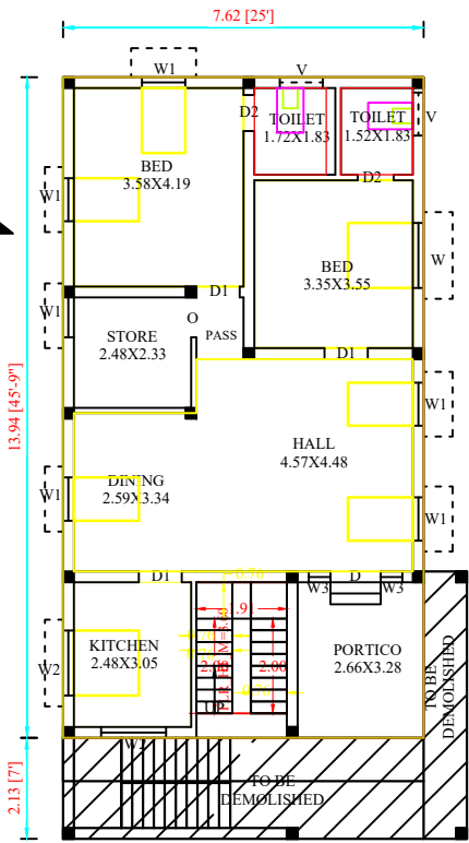
EXIS. GROUND FLOOR PLAN
