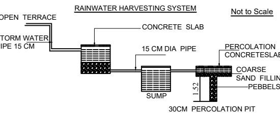
30CM PERCOLATION PIT
