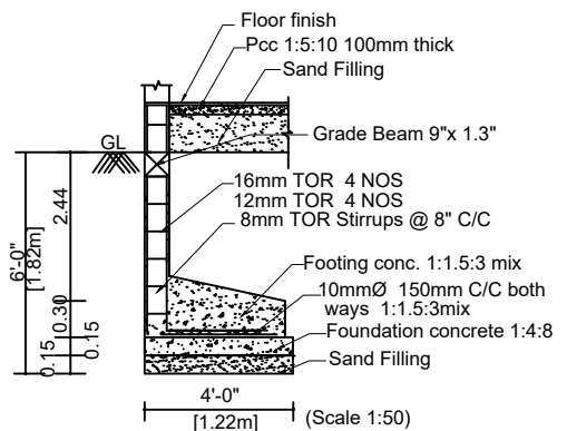
FOUNDATION DETAILS
