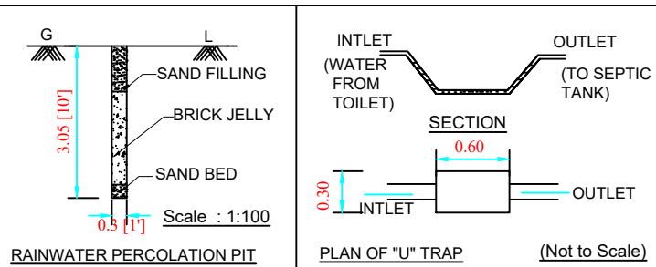
RAINWATER PERCOLATION PIT
