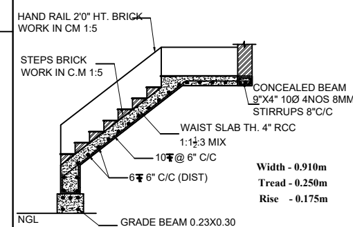
STAIRCASE DETAILS
