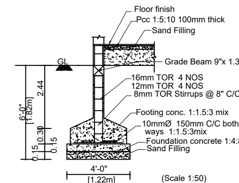
FOUNDATION DETAILS
