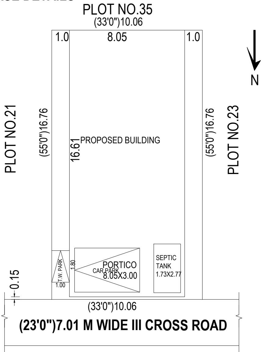
SITE PLAN
