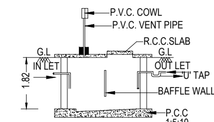
SEC. OF SEPTIC TANK"AA"
