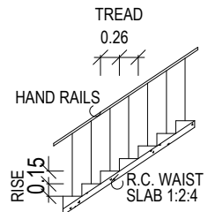
STAIRCASE DETAILS
