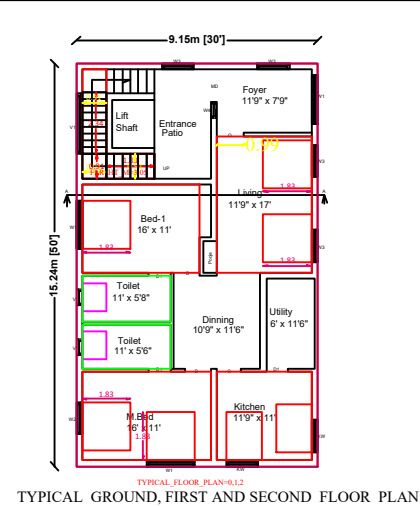
TYPICAL GROUND, FIRST AND SECOND FLOOR PLAN
