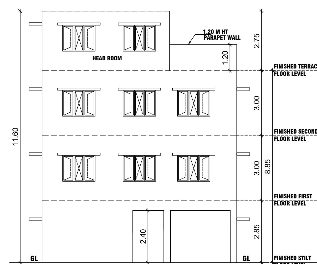
FRONT ELEVATION
