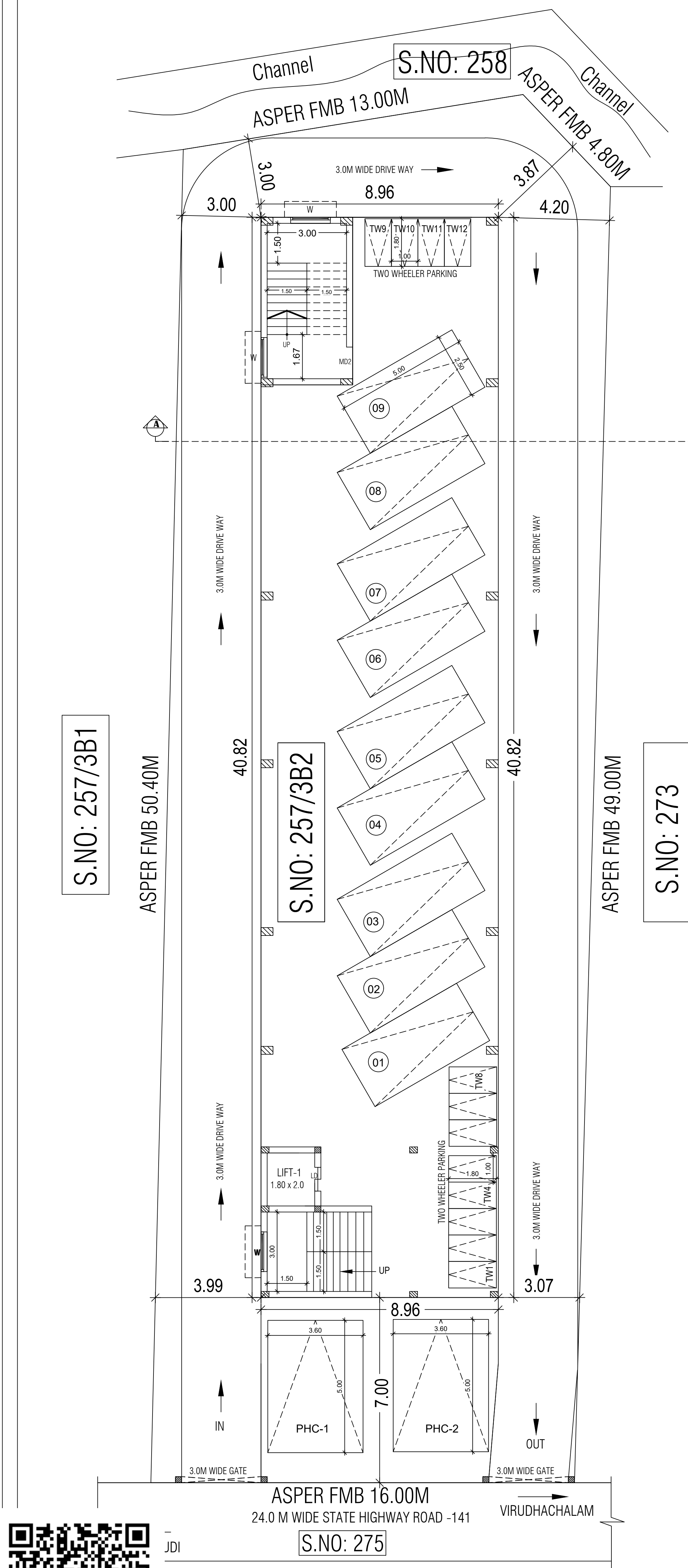
SITE CUM STILT FLOOR PLAN
