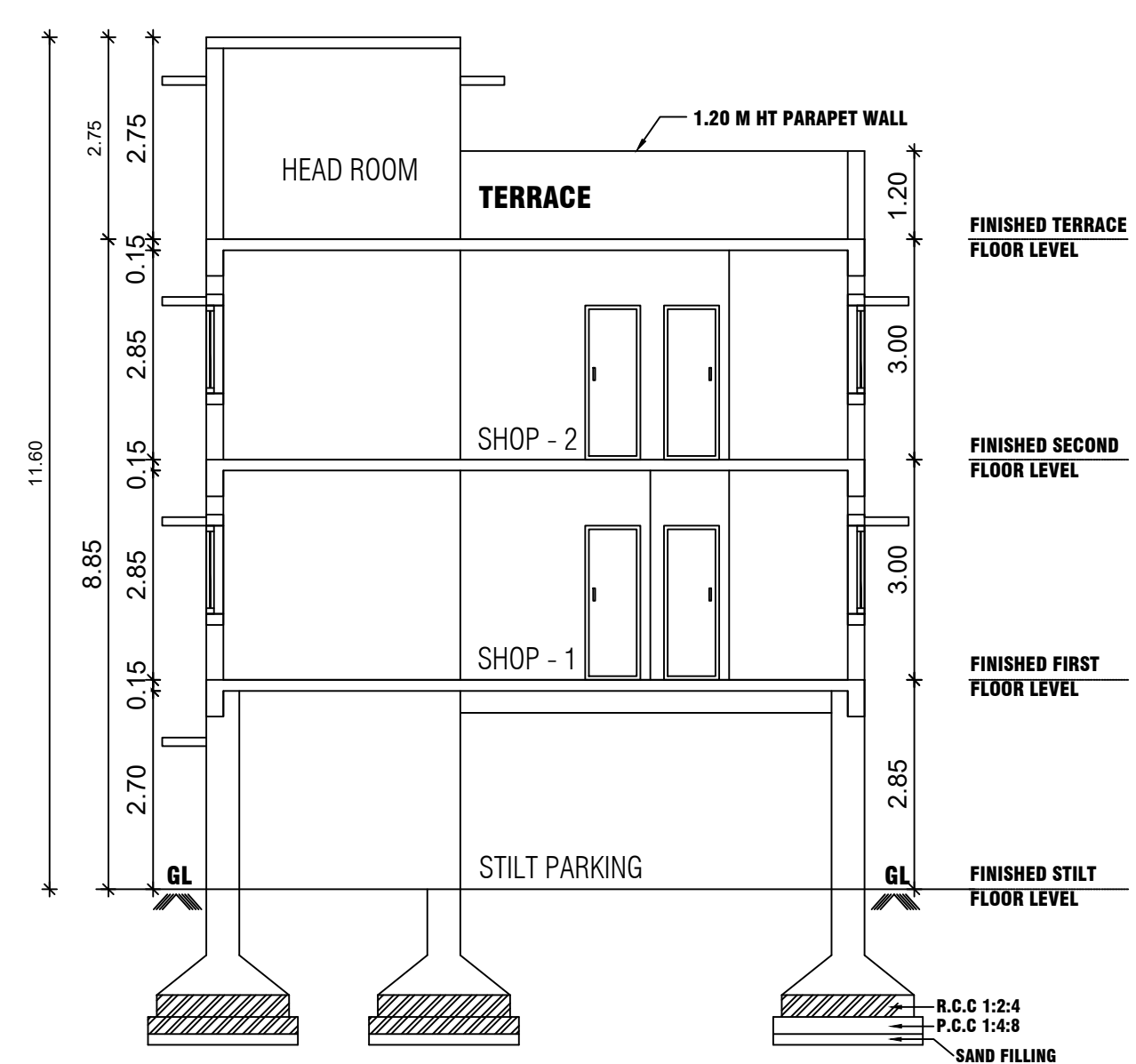
SECTION - "AA"
