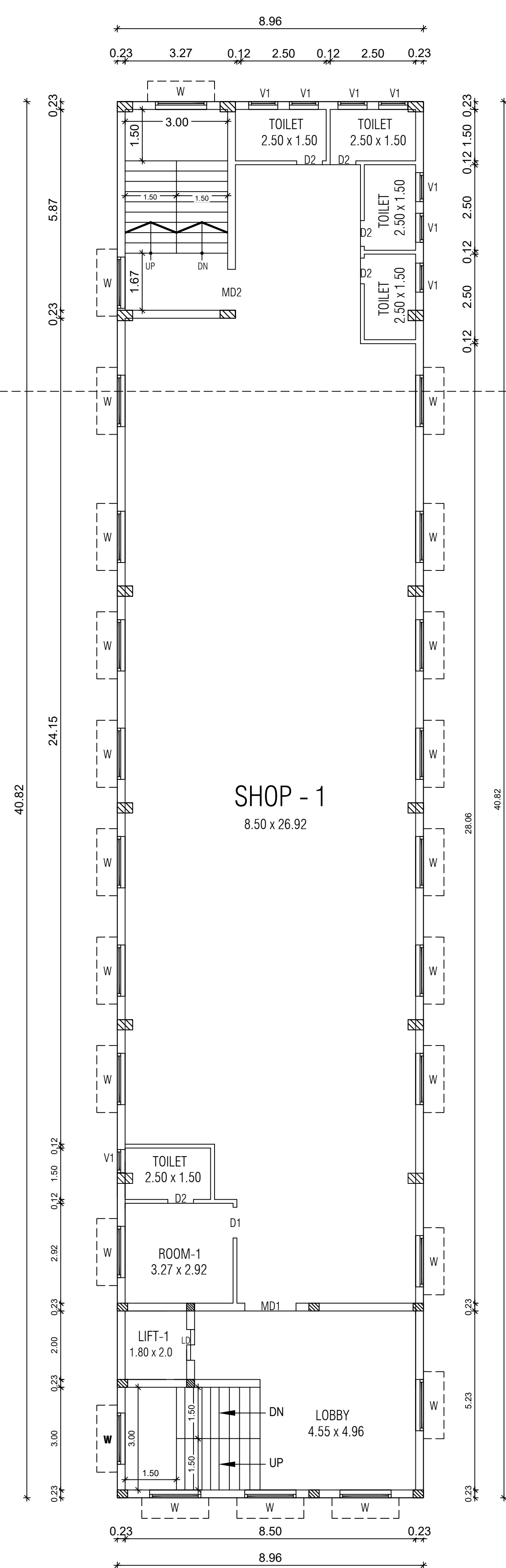
TYPICAL FIRST & SECOND FLOOR PLAN
