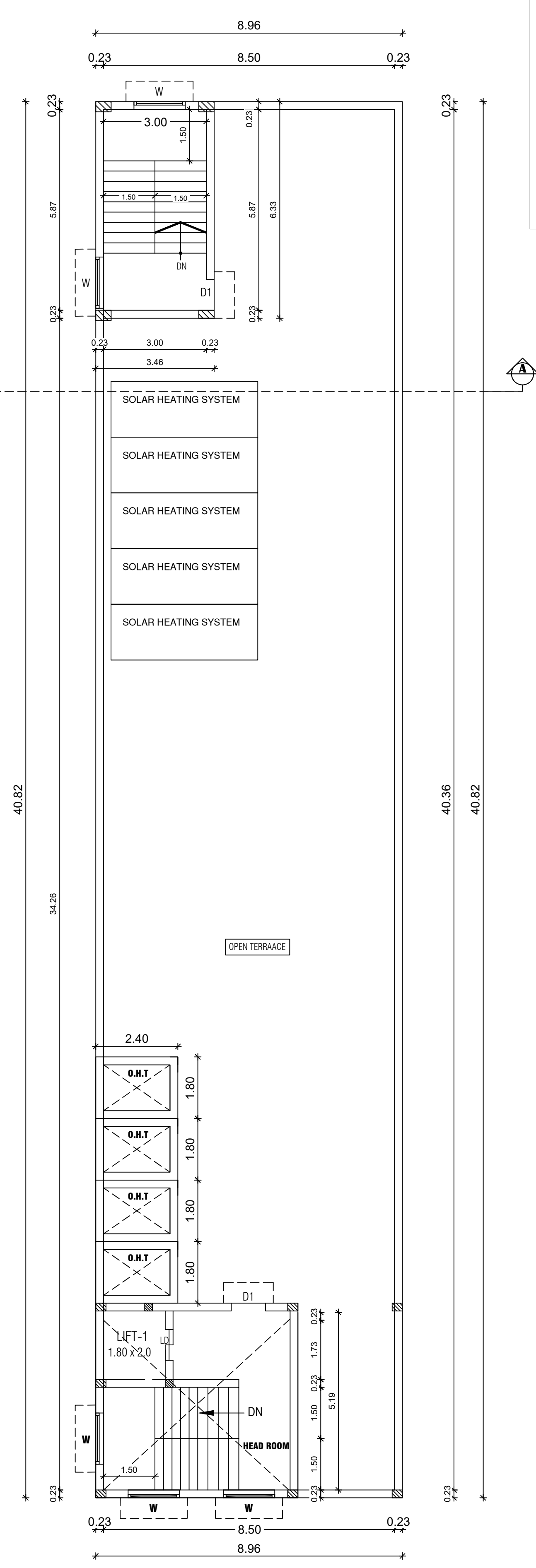
TEERACE FLOOR PLAN
