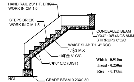
STAIRCASE DETAILS (Scale 1:50)
