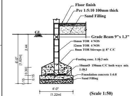
FOUNDATION DETAILS
