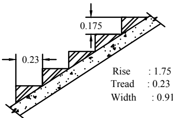
STAIRCASE DETAILS
