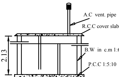
SECTION
