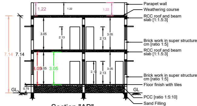
Section "AB"
