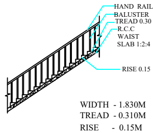
STAIR CASE DETAILS (SCALE 1:100)
