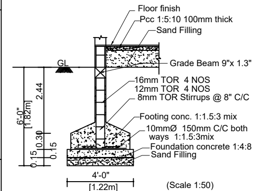
FOUNDATION DETAILS
