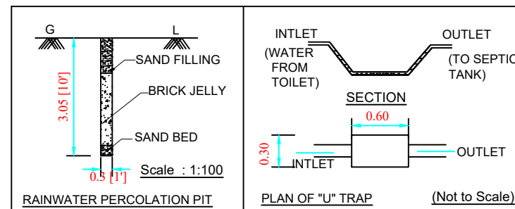
RAINWATER PERCOLATION PIT
