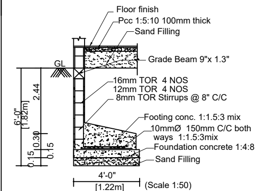
FOUNDATION DETAILS
