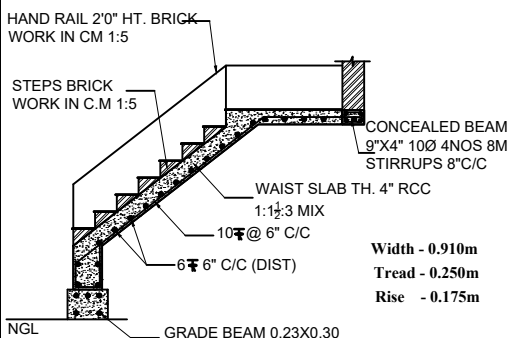
STAIRCASE DETAILS
