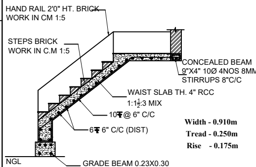
STAIRCASE DETAILS
