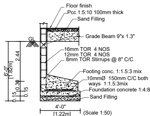
FOUNDATION DETAILS
