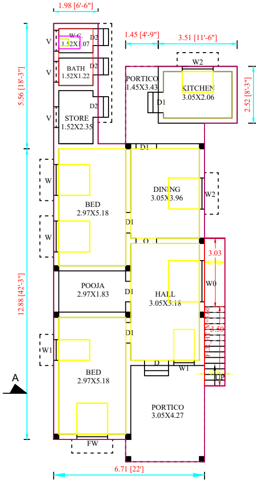
EXIS.GROUND FLOOR PLAN
