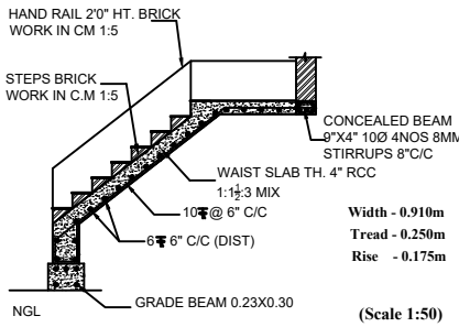
STAIRCASE DETAILS
