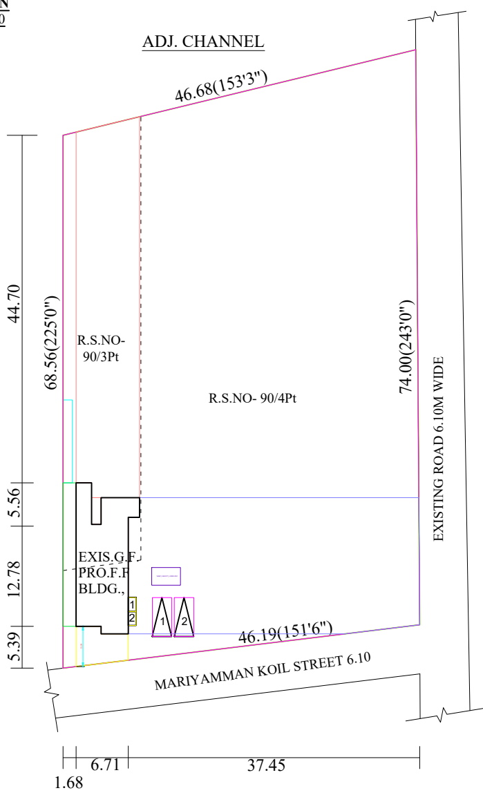
RAINWATER HARVESTING SYSTEM
