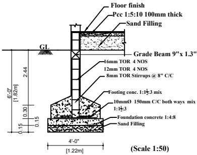
FOUNDATION DETAILS
