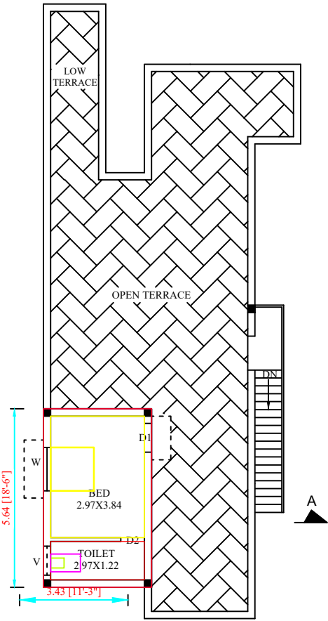
PRO.ADD.FIRST FLOOR PLAN
