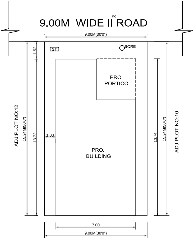
SITE PLAN
