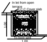
RAIN WATER HARVESTING
