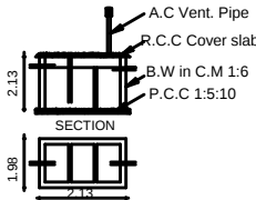
SEPTICTANK
