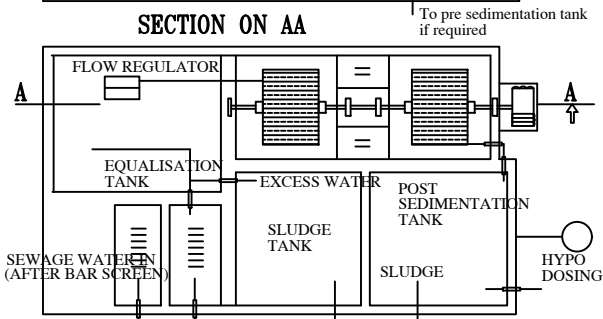
SECTION ON AA PLAN SEWAGE TREATMENT PLANT DETAILS WASTE WATER RECYCLING UNIT
