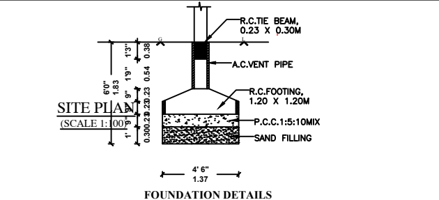
FOUNDATION DETAILS
