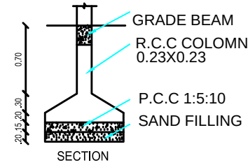
FOUNDATION DETAILS
