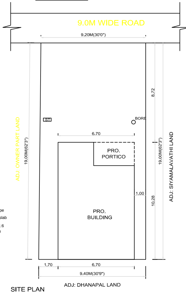
SITE PLAN
