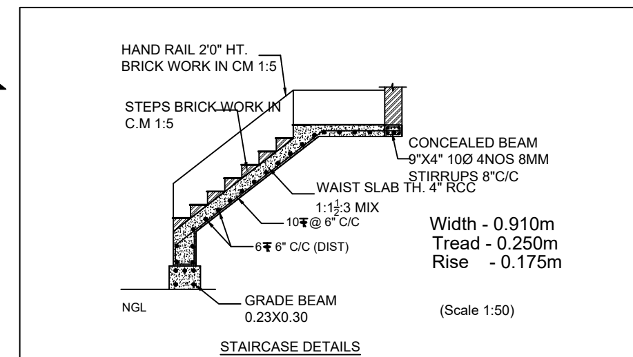
STAIRCASE DETAILS
