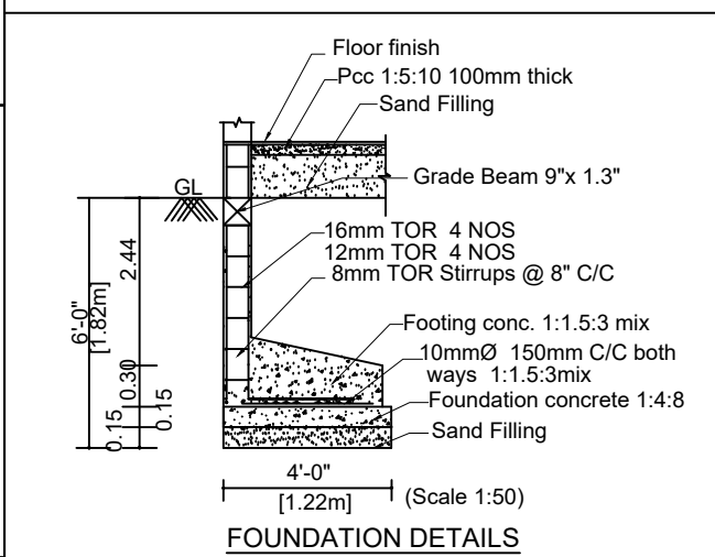
FOUNDATION DETAILS
