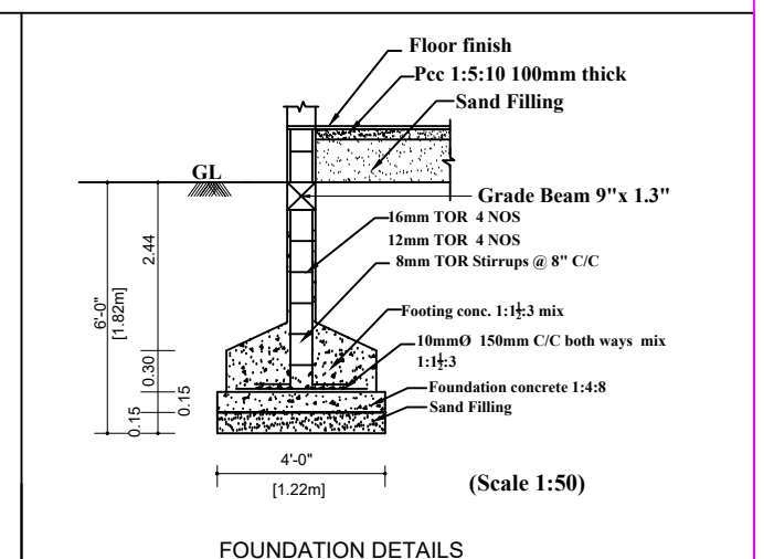
FOUNDATION DETAILS
