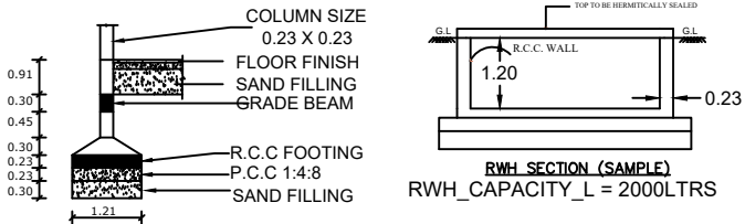
FOUNDATION DETAILS SCALE 1:500
