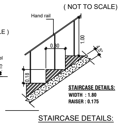
STAIRCASE DETAILS:
