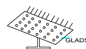
SOLAR SYSTEM
