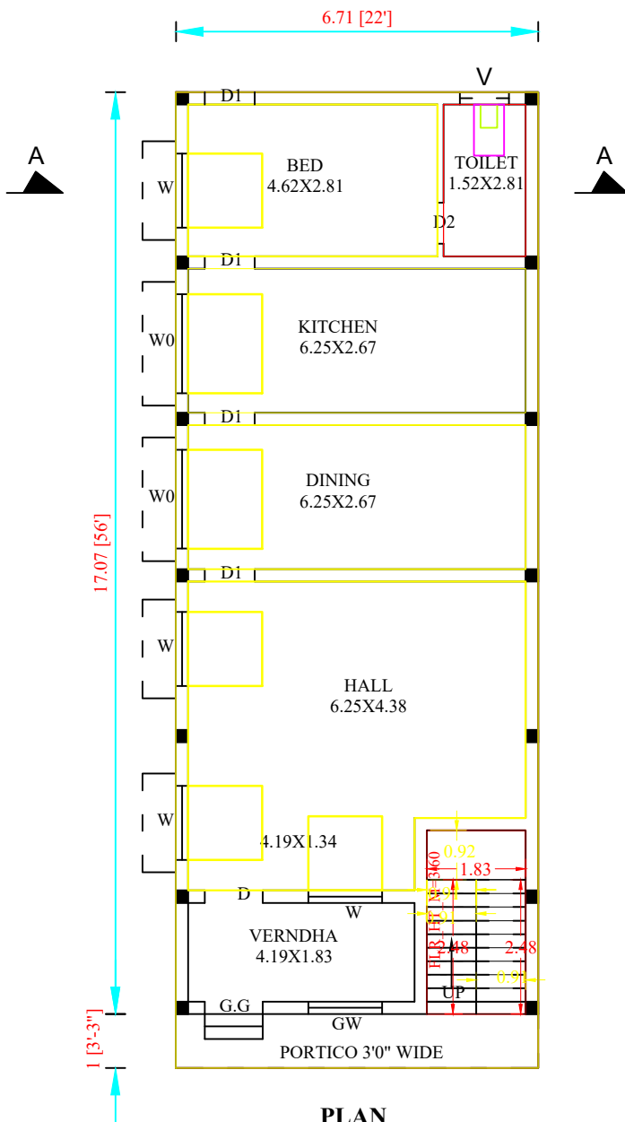
PLAN
