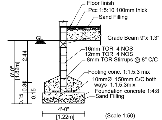
FOUNDATION DETAILS
