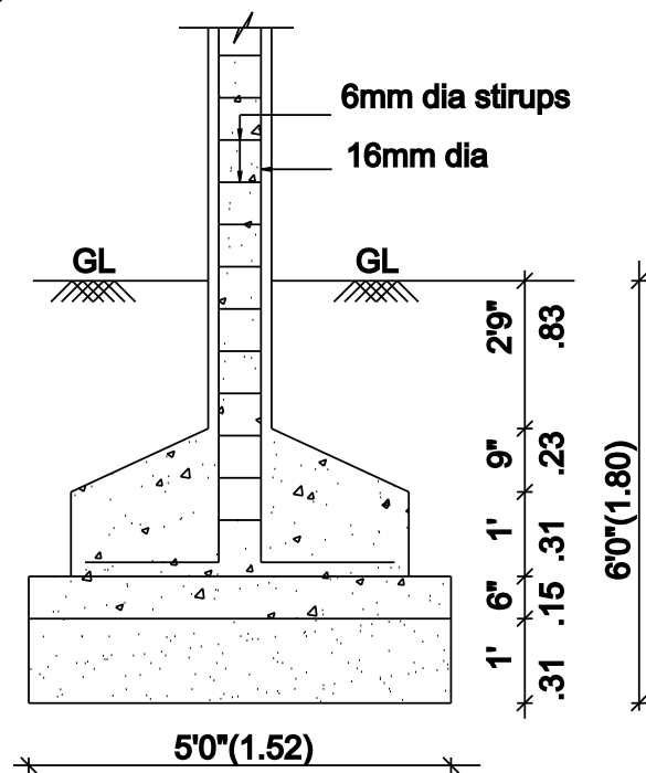
FOUNDATION DETAIL
