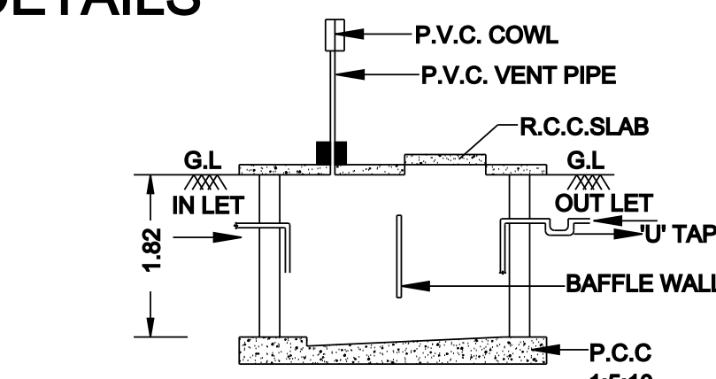
SEC. OF SEPTIC TANK"AA"
