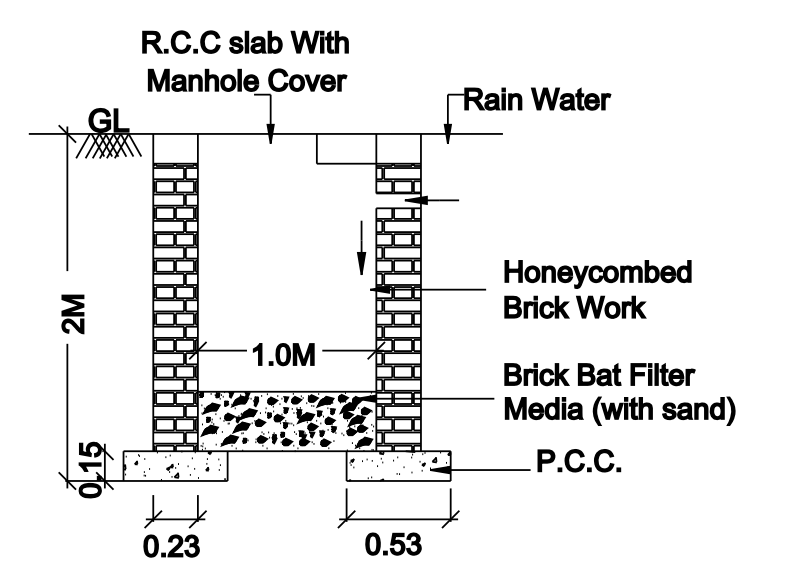
DETAILS OF RAIN WATER COLLECTION PIT SCALE:- 1"=4'0"
