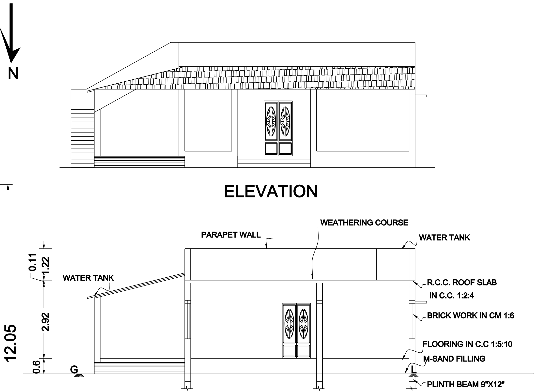
SECTION AT 'AB'
