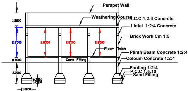
Section Section - AA
