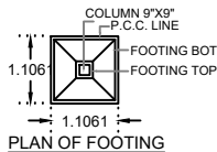
PLAN OF FOOTING
