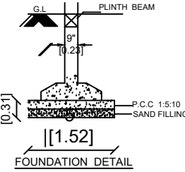
FOUNDATION DETAIL
