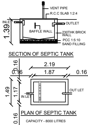
CAPACITY - 8000 LITRES
