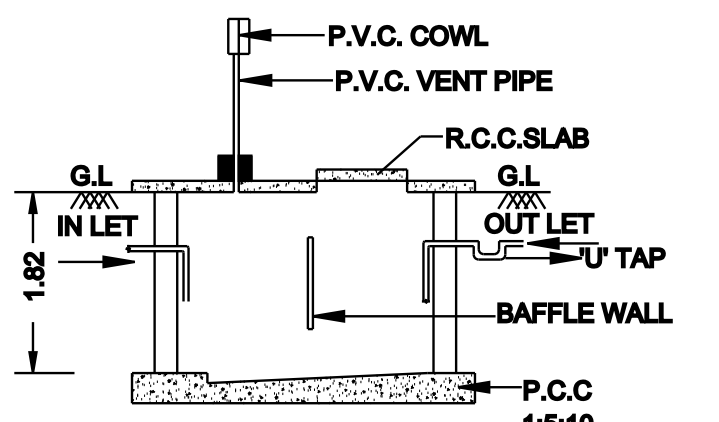
SEC. OF SEPTIC TANK
