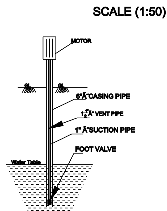
SEC. OF BOREWELL
