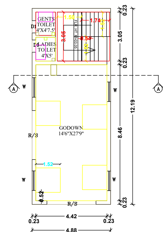
PROPOSED GROUND FLOOR PLAN (BUILDING-2)
