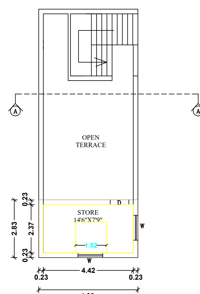
PROPOSED FIRST FLOOR PLAN (BUILDING-2)
