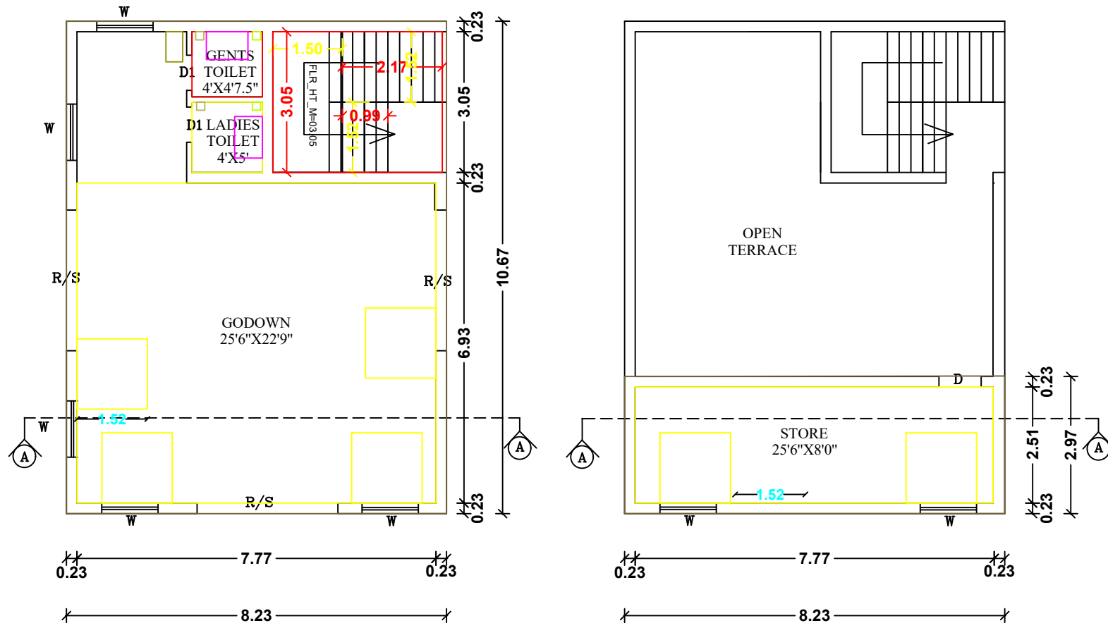
PROPOSED GROUND FLOOR PLAN (BUILDING-1)
