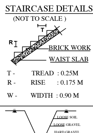
STAIRCASE DETAILS
