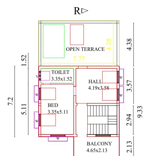
FIRST_FLOOR_PLAN=1 FIRST FLOOR PLAN
