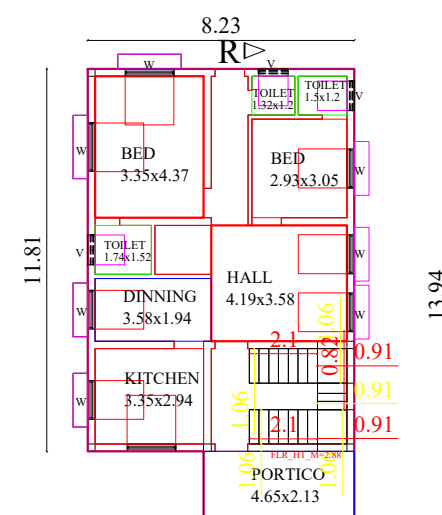
GROUND_FLOOR_PLAN=0 GROUND FLOOR PLAN
