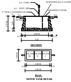
SEPTIC TANK DETAIL
