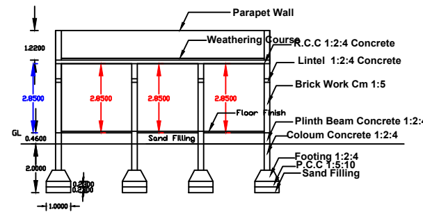
Section Section - AA
