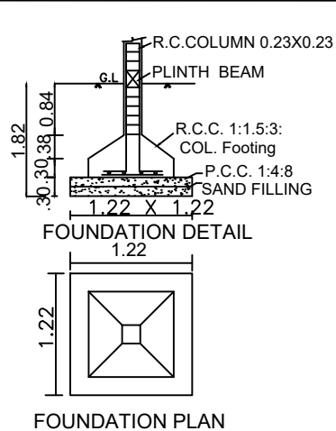
FOUNDATION PLAN
