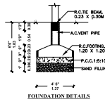
FOUNDATION DETAILS
