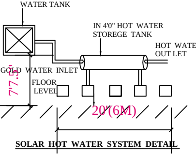
SOLAR HOT WATER SYSTEM DETAIL
