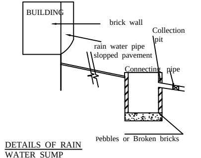
DETAILS OF RAIN WATER SUMP
