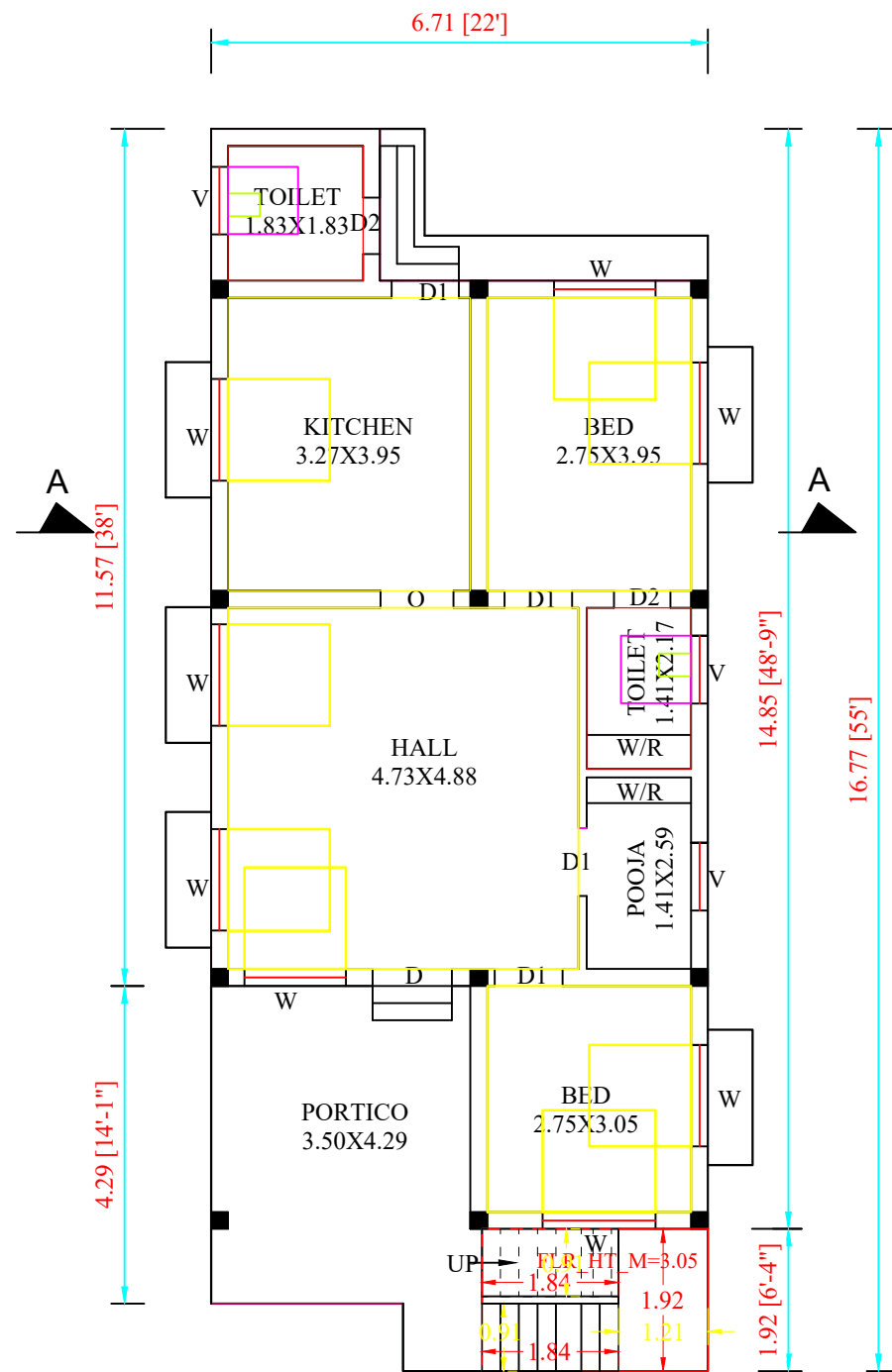
PLAN
