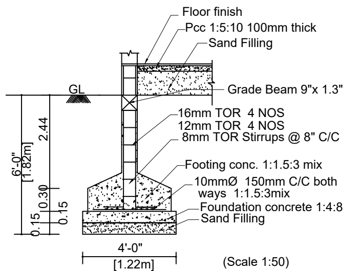
FOUNDATION DETAILS
