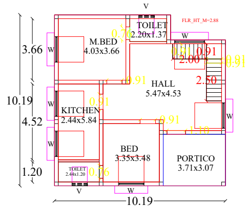
GROUND_FLOOR_PLAN=0 GROUND FLOOR PLAN
