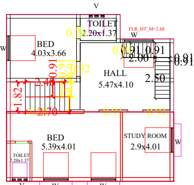
FIRST_FLOOR_PLAN=1 FIRST FLOOR PLAN
