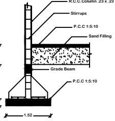
COLUMN DETAIL
