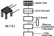
SOLAR SYSTEM FLOW DIAGRAM
