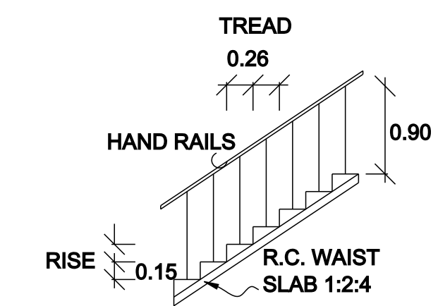
STAIRCASE DETAILS
