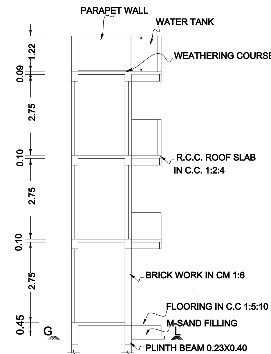
SECTION AT 'AB'
