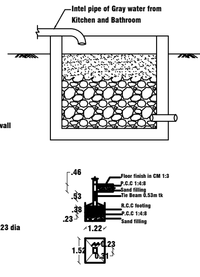
GREY WATER RECYCLING CHAMBER:-
