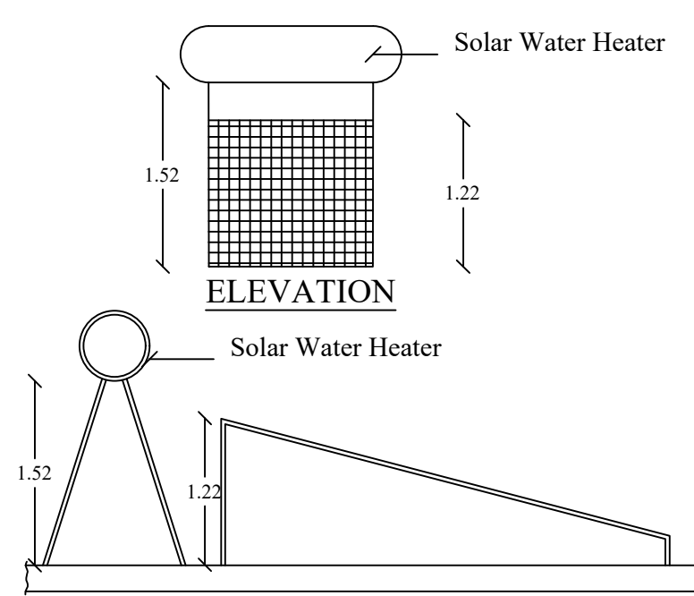
SOLAR WATER HEATER DETAILS
