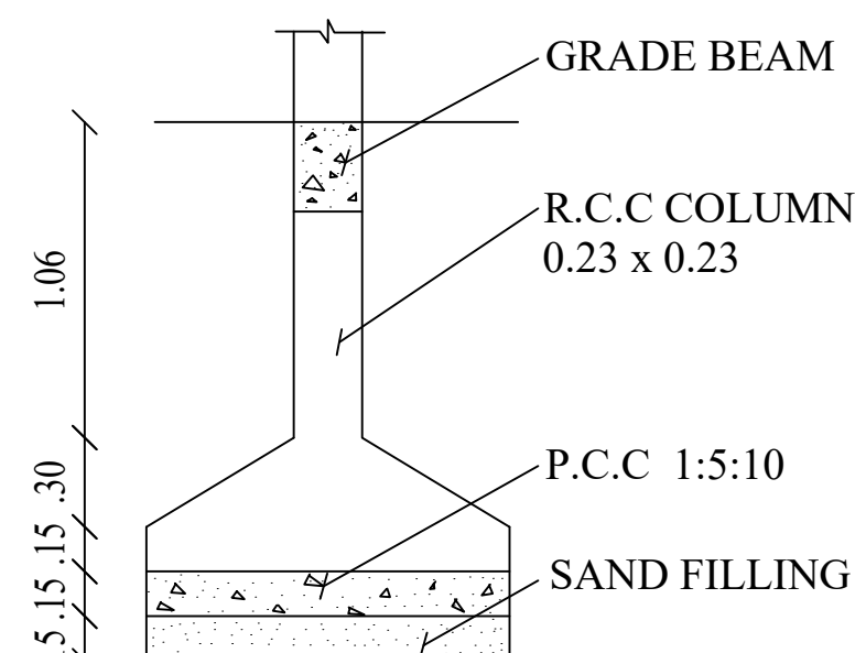
SECTION 1.22 0.61 0.305 PLAN FOUNDATION DETAILS
