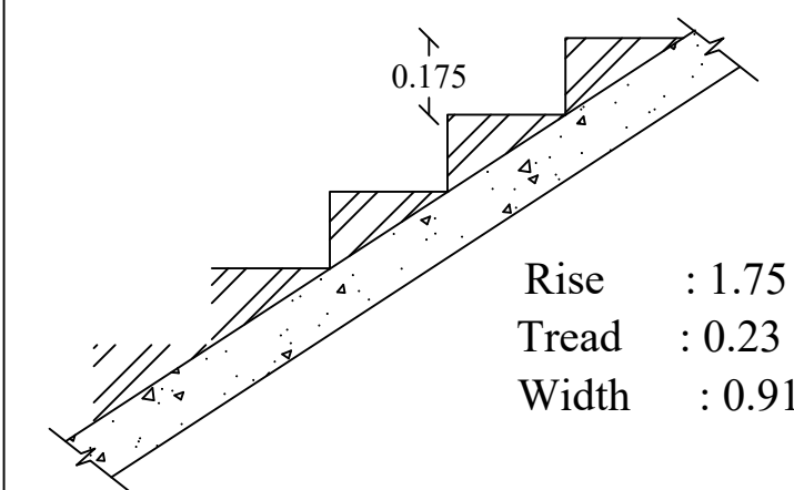
STAIRCASE DETAILS
