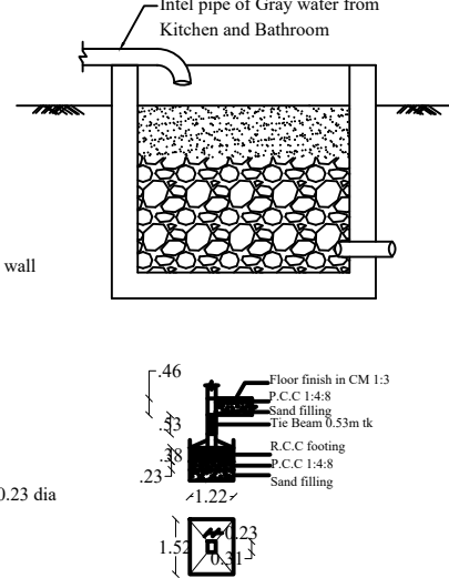
GREY WATER RECYCLING CHAMBER:-
