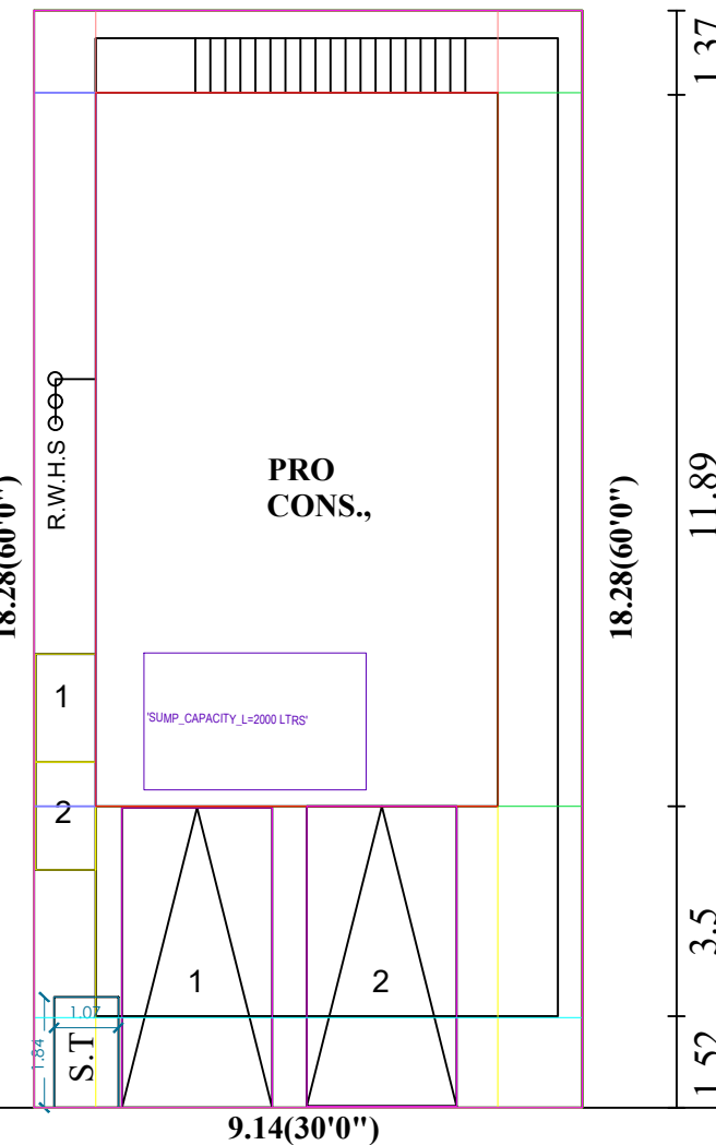
LAYOUT ROAD 6.1M WIDE
