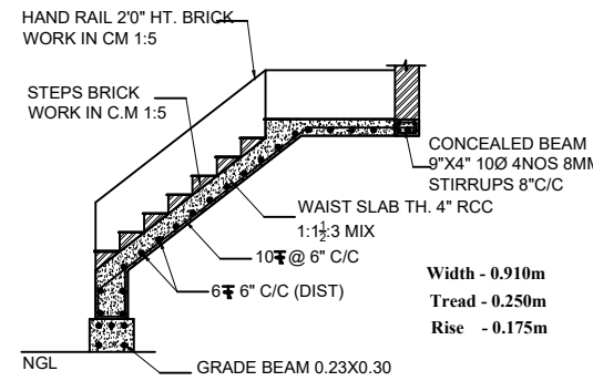
STAIRCASE DETAILS
