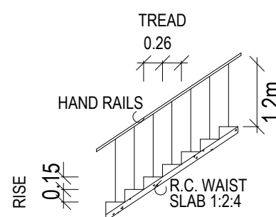
STAIRCASE DETAILS
